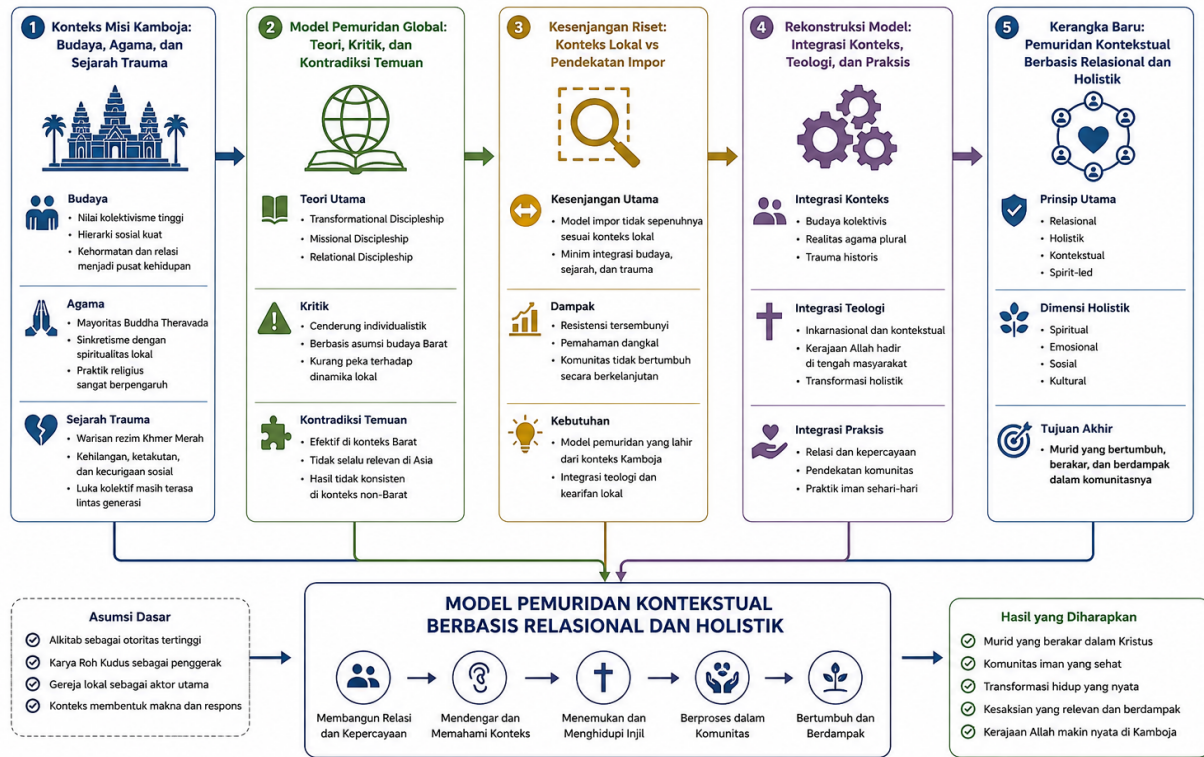
Gambar 1. Conceptual Framework
